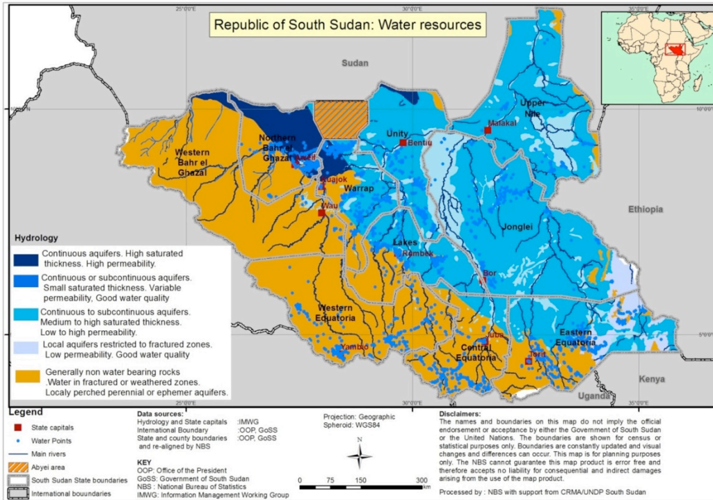
Figure 1.3: Geological Information
